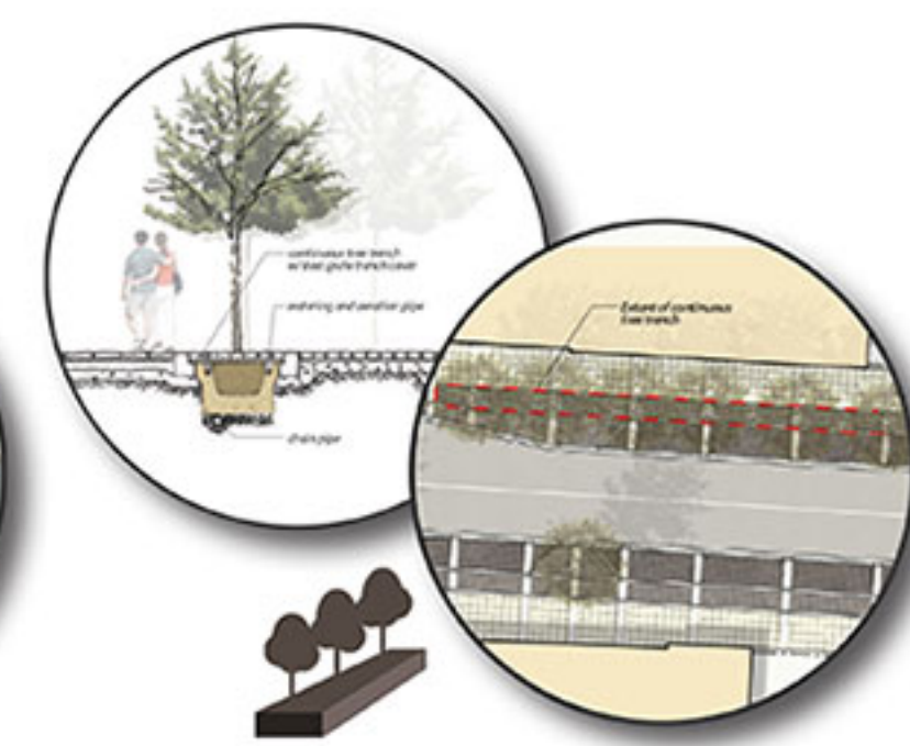
CONTINUOUS TREE TRENCH SYSTEM
